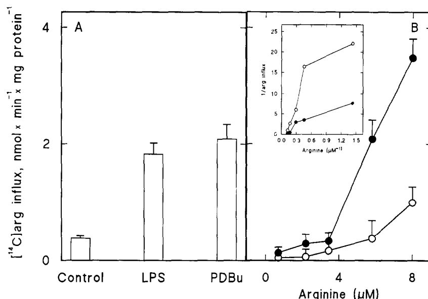
Fig. 2. Effect of PDBu on arginine influx. Macrophages ( 2 \times 10^6 ) were incubated with 100 nM PDBu or 50 \mu\text{g}/\text{ml} of LPS for 4 h and the transport of [\text{U-}^{14}\text{C}]\text{arginine} (5 \mu\text{M} ) was measured (panel A). The rate of arginine influx was calculated by the measurement of the radioactivity incorporated at 30 and 60 s. The dose-dependent influx was assayed in unstimulated (○) or 4-h treated cells with 100 nM PDBu (●) (panel B). The inset shows the Lineweaver-Burk plot for the arginine uptake corresponding to the data given in panel B. Results are means \pm S.E.M. of 3 independent determinations.
